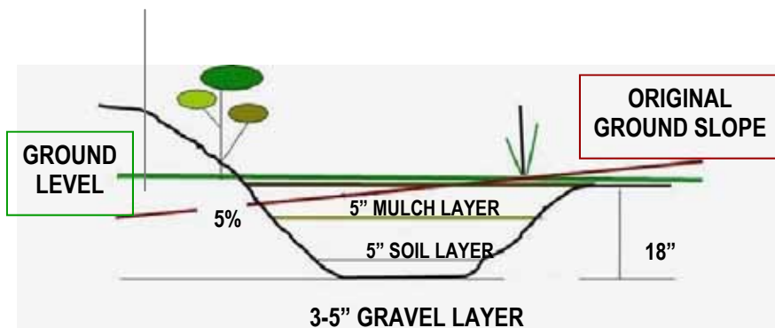
Cross-section of a rain garden
